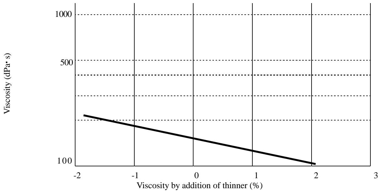
Fig.2 Relationship between viscosity and addition of thinner MC-192
