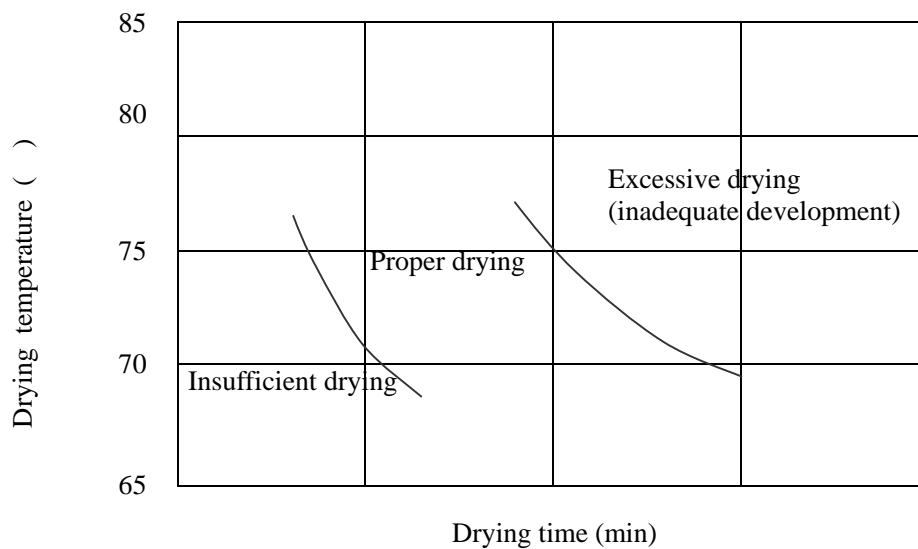
Fig.3 Pre-drying temperature, drying time and the dried condition of the film
