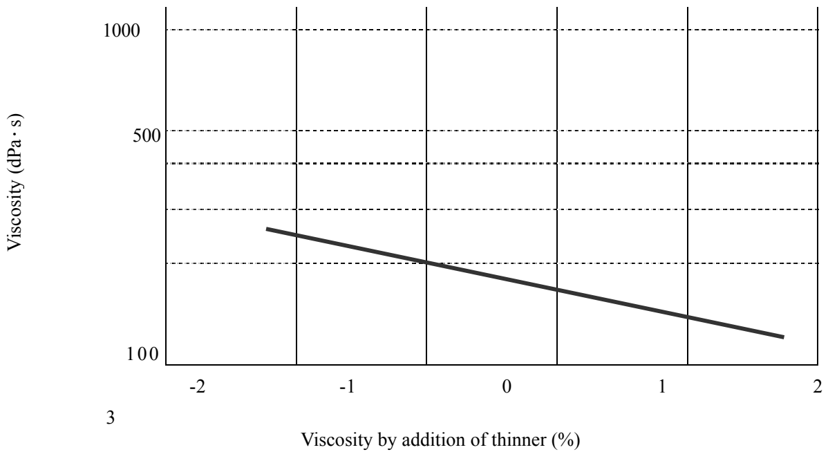
Fig.2 Relationship between viscosity and addition of thinner #313
