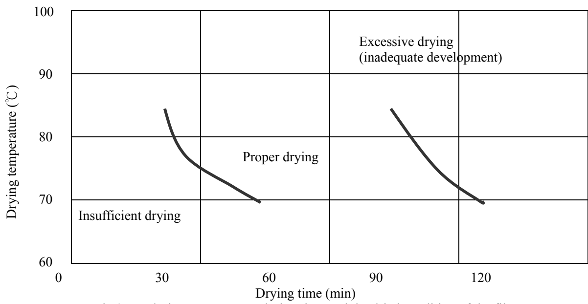
Fig.3 Pre-drying temperature, drying time and the dried condition of the film
